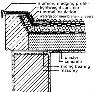
9 Protective layer – double layer gravel bedding; better: ballasting
